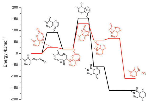
Fig. 1 Energy surface for the formation of compounds 22 and 24 .
