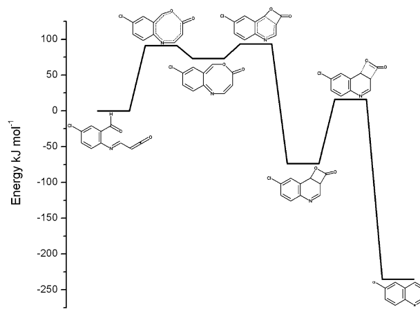
Fig. 2 Energy surface for the formation of 6-chloroquinoline 30 .
